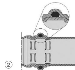
Cross section of a pressed connector.
